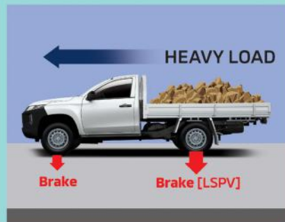
Load Sensing Proportioning Valve [LSPV] (Cab & Chassis)
